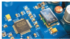
ESS ES9038PRO (左)とCCHD-957(右)
